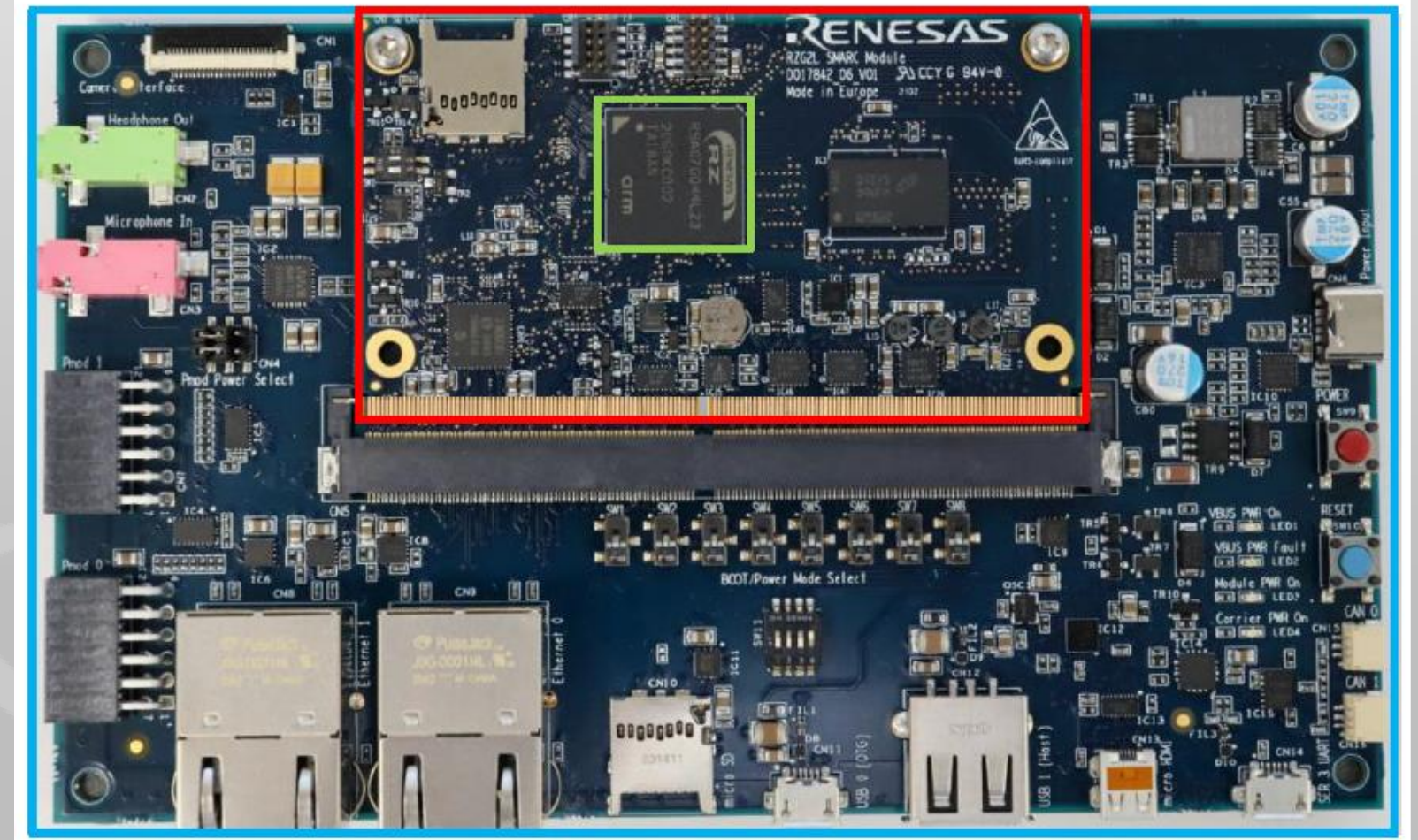
RZ/G2L SMARC v2.1 Module board + Carrier Board (Made by Renesas Europe)
